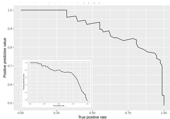
Supplementary Figure 4: Performance curves for each respective model where the outer graph are results from the test curve, and the inner curve is aggregated performance from the K-fold cross validation.
